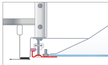
Compatible with both drywall and grid ceilings.
